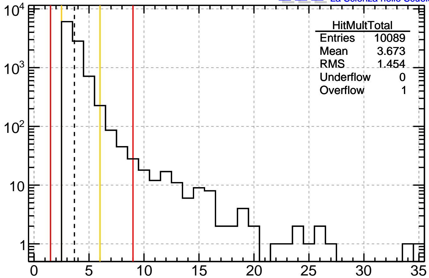
Hit multiplicity Total
